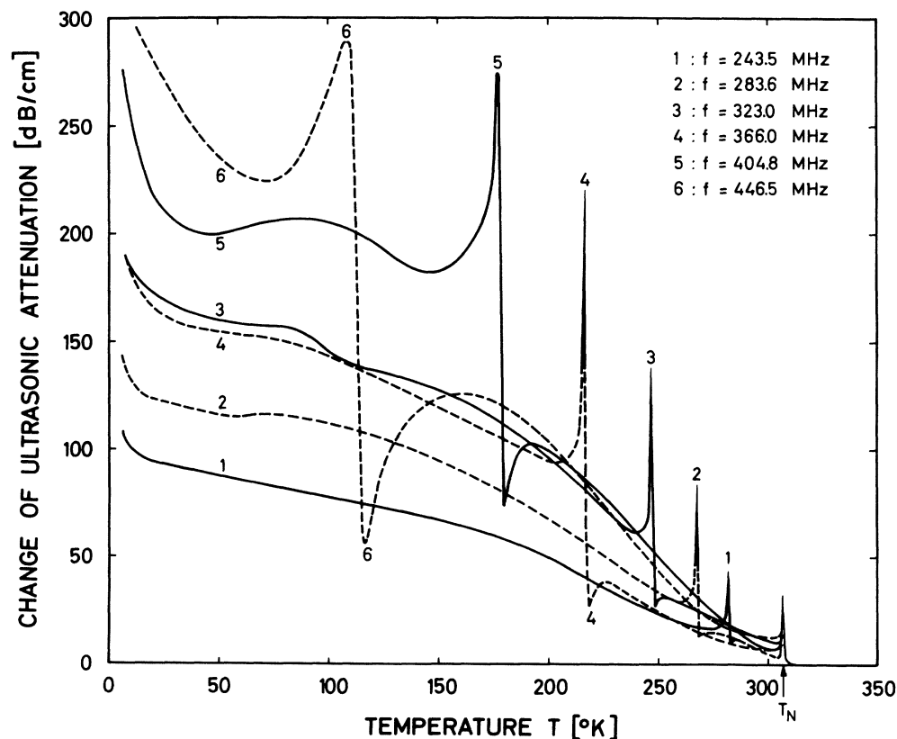
FIG. 1. Temperature dependence of ultrasonic attenuation for a longitudinal wave in MnTe at H=0 ( f=243.5 to 446.5 MHz).
