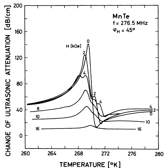
FIG. 8. Temperature dependence of ultrasonic attenuation for a longitudinal wave with q \parallel x , f=276.5 MHz in MnTe. Magnetic field H as parameter, \varphi_H=45^\circ .
